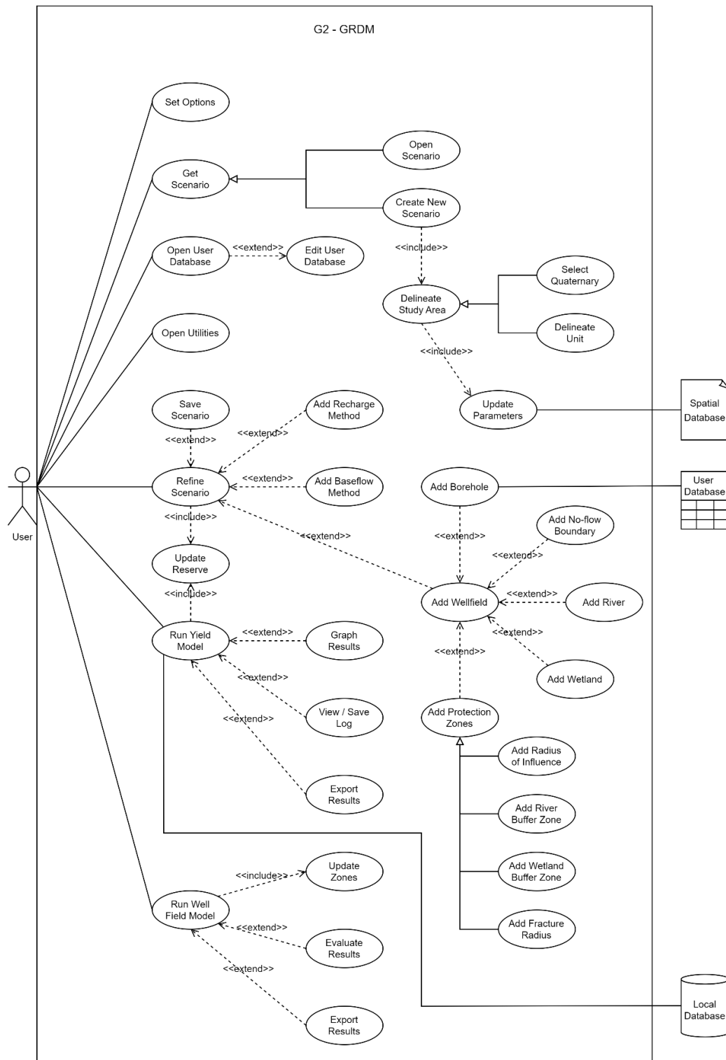
Figure 7: G2 Use Case Diagram (excluding Spatial and Monitoring functionality)
