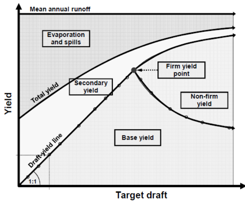
Figure 19: Target draft vs. yield diagram
